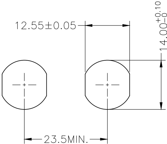
PANEL HOLE
