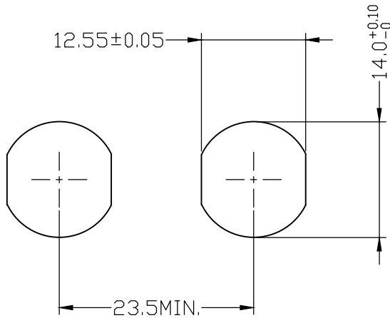
PANEL HOLE
